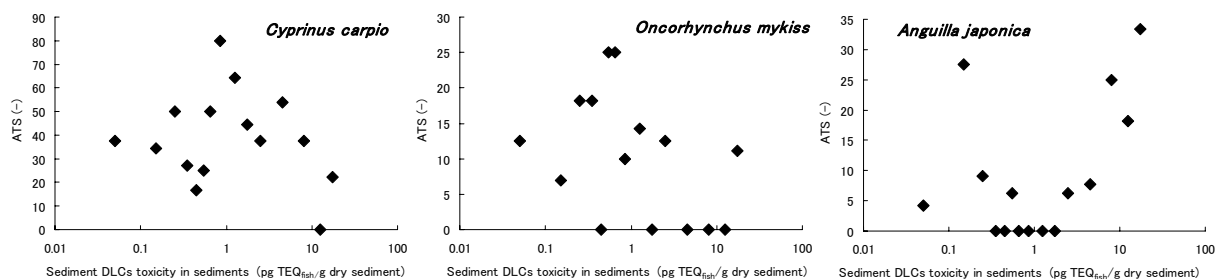
Fig. 2 The relationship between DLCs toxicity in sediments and “Appearance of Target Species (ATS)” for each 5 species
